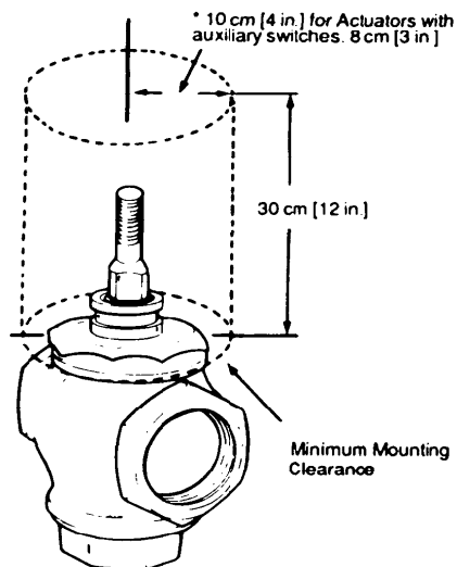
FIG. 2 -- MINIMUM MOUNTING CLEARANCE.
